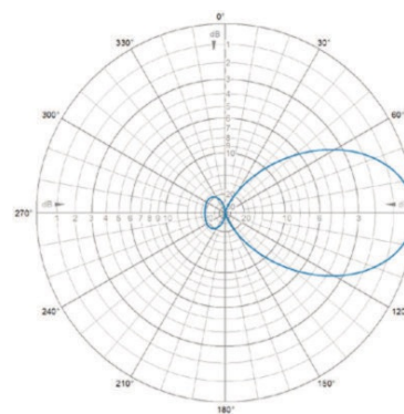
E-Plane | 405 MHz
